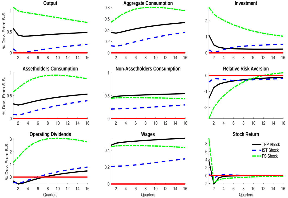
Figure D.2: Conditional dynamics - Additional variables
