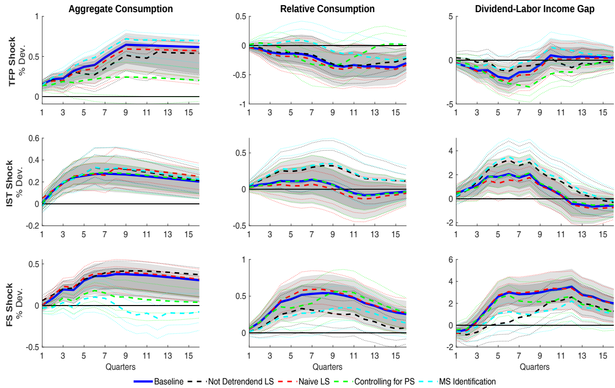
Figure E.4: Empirical conditional dynamics - Mechanism - Robustness
